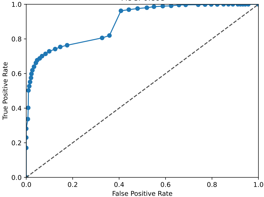
JUNB ROC Curve AUC: 0.895
