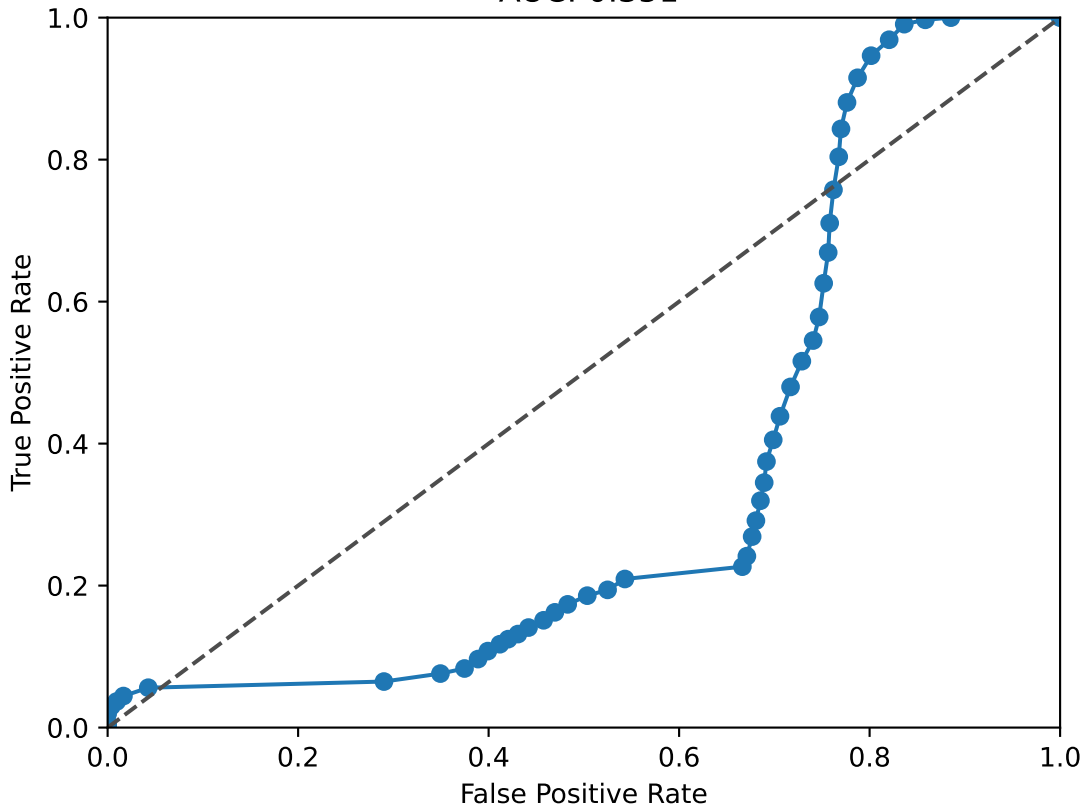
NFIB ROC Curve AUC: 0.351
