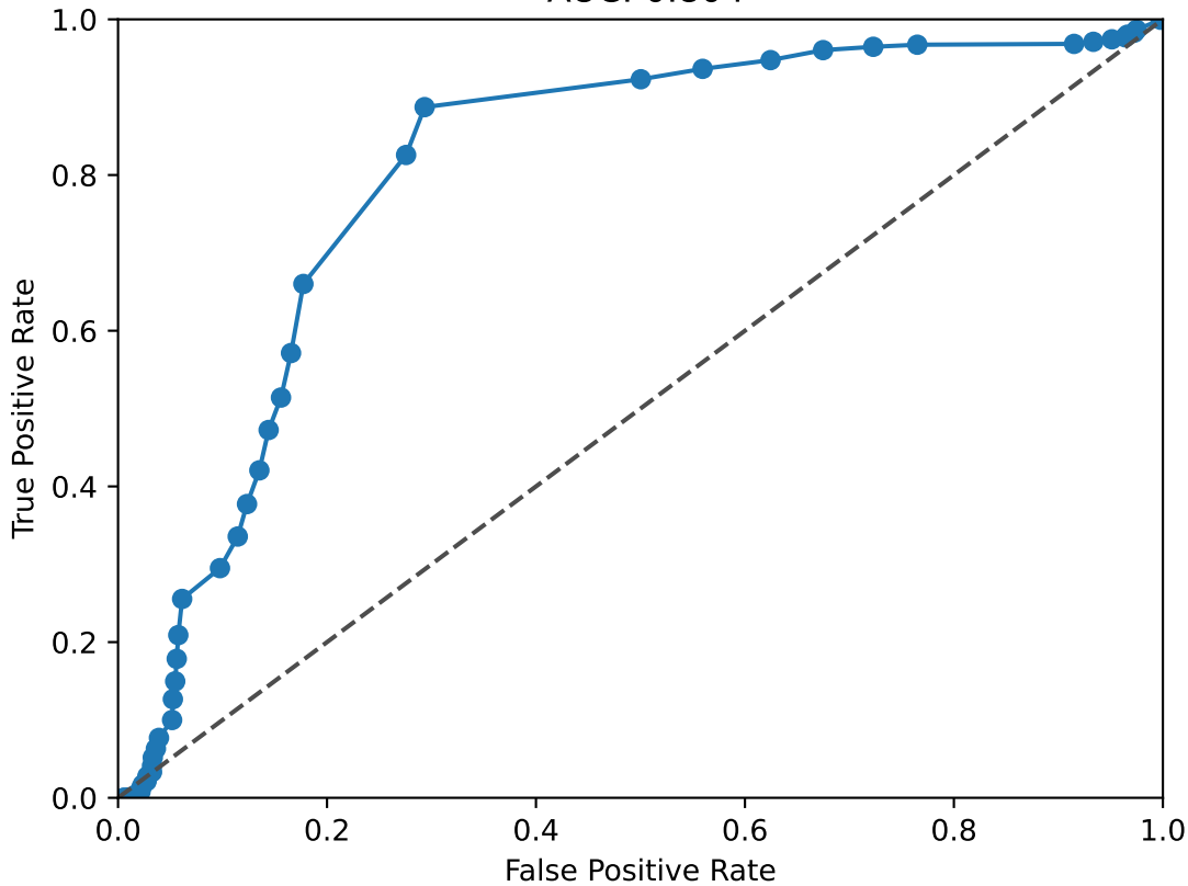
NFIX ROC Curve AUC: 0.804
