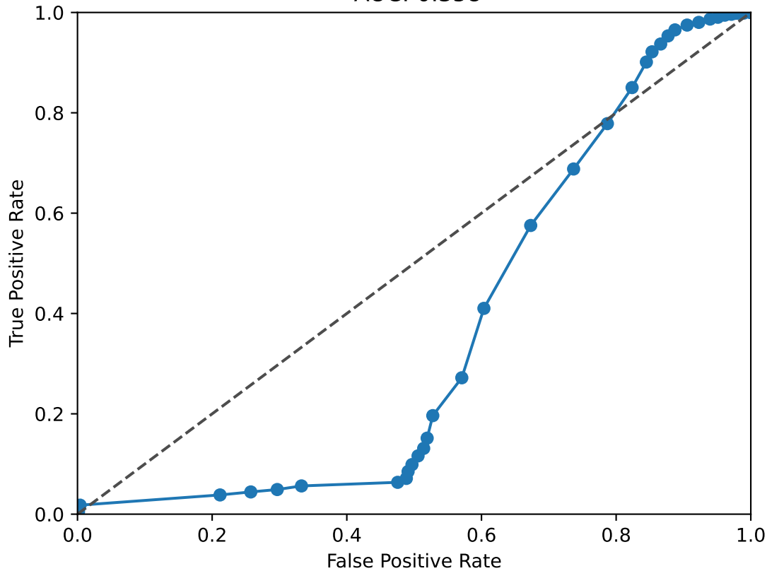
PBX1 ROC Curve AUC: 0.358
