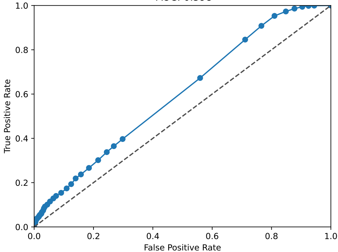
PROX1 ROC Curve AUC: 0.598
