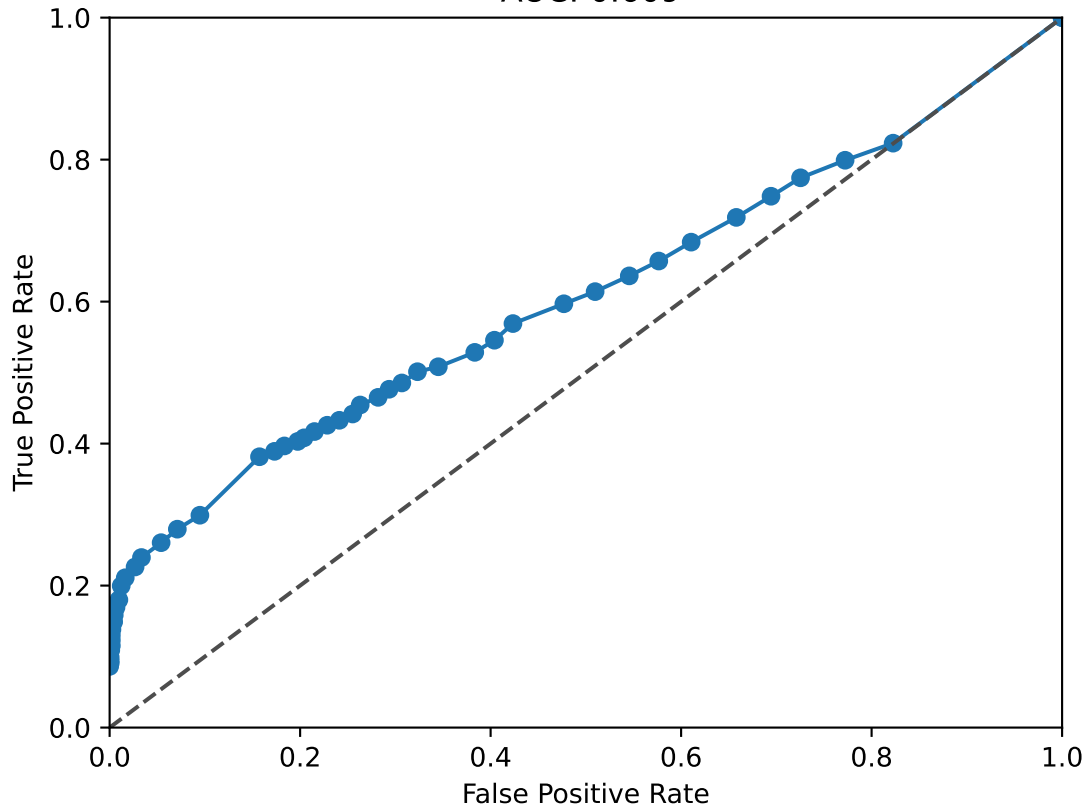
REST ROC Curve AUC: 0.609
