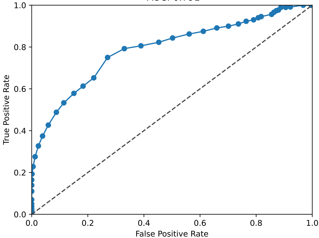
SIX4 ROC Curve AUC: 0.791
