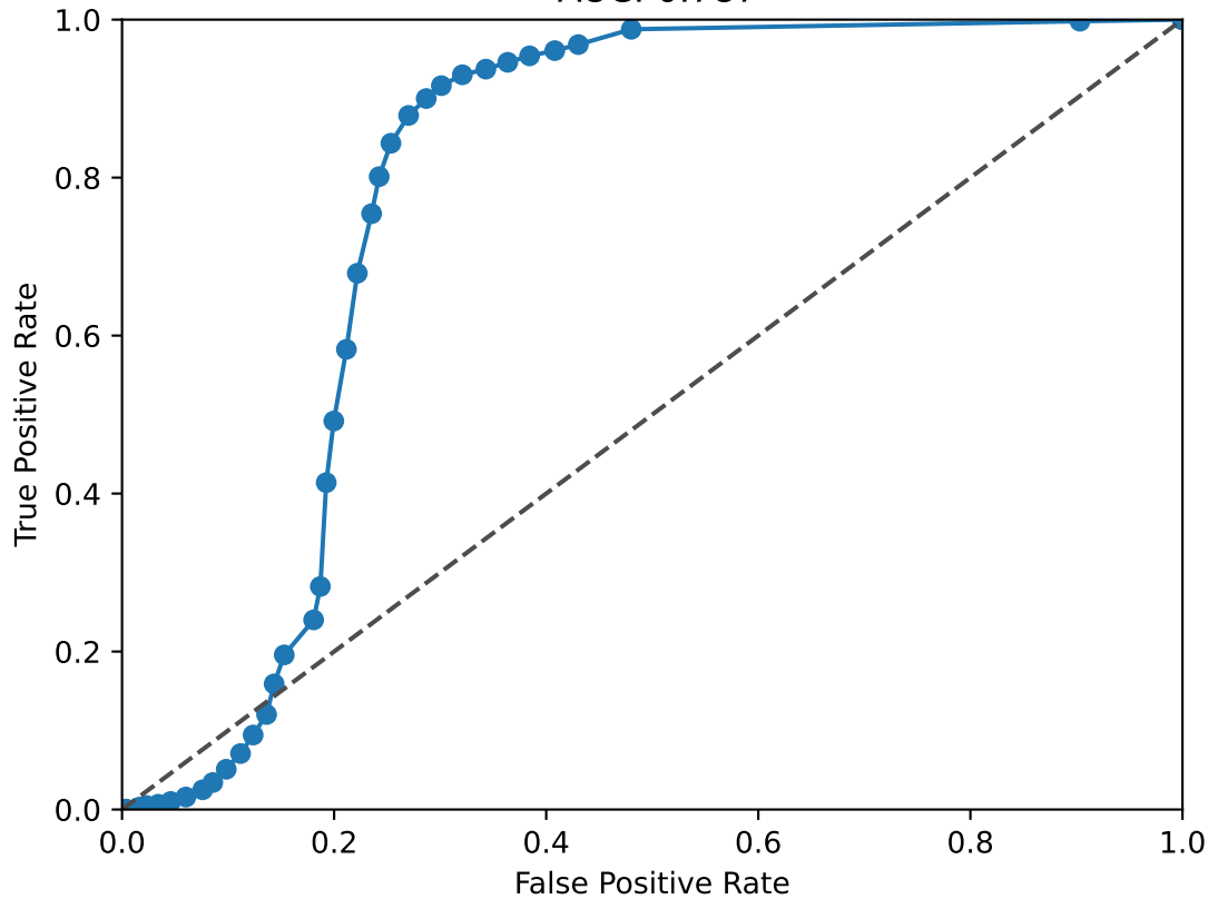
SOX11 ROC Curve AUC: 0.787
