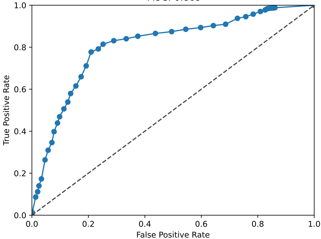
STAT2 ROC Curve AUC: 0.809
