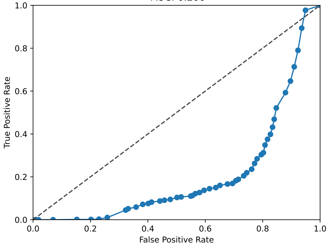
ASCL1 ROC Curve AUC: 0.206
