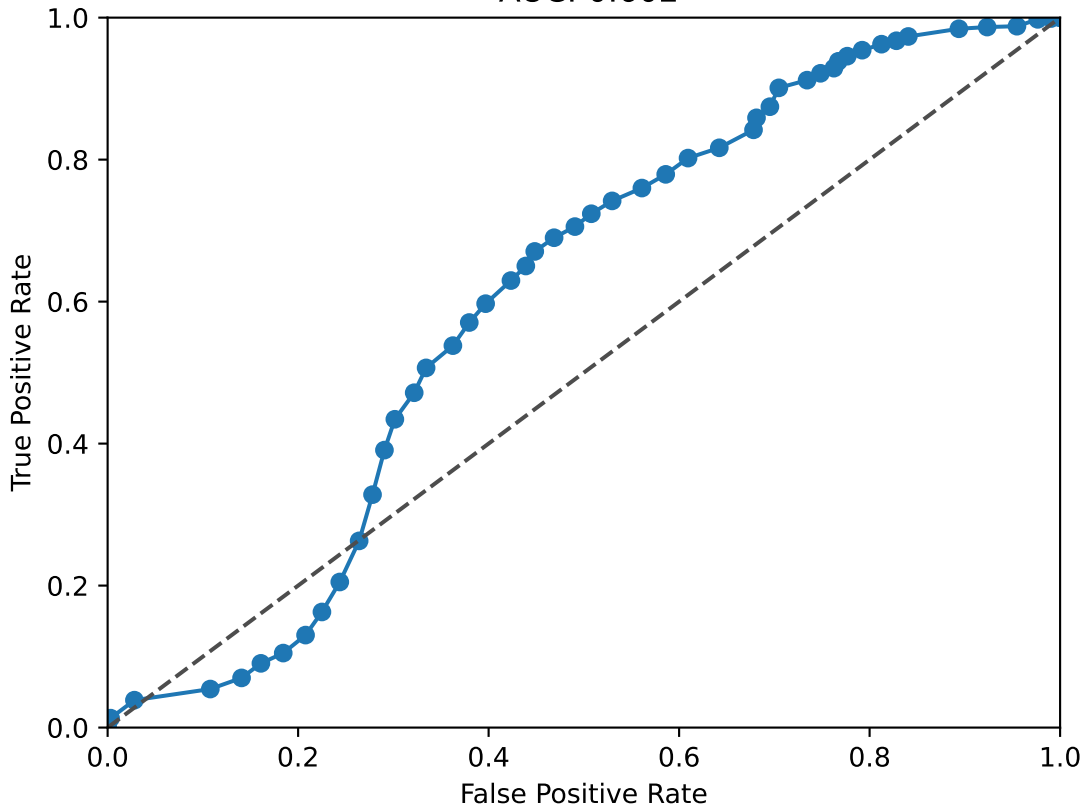
EPCAM ROC Curve AUC: 0.602
