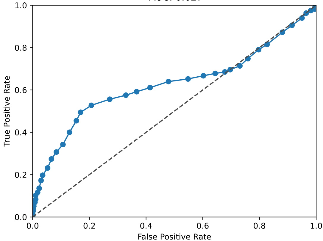
FOS ROC Curve AUC: 0.627
