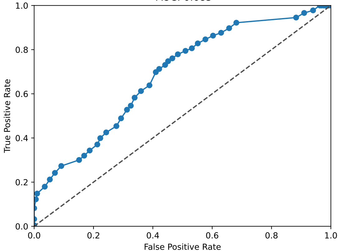
LMX1B ROC Curve AUC: 0.685
