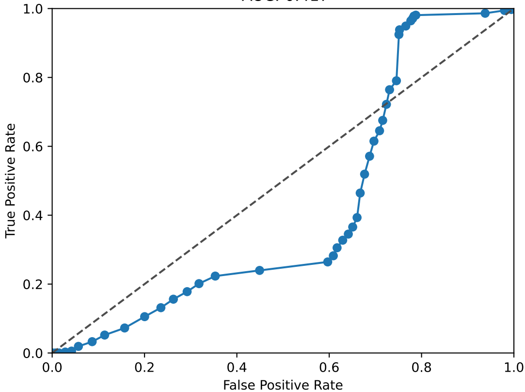
NFATC2 ROC Curve AUC: 0.417
