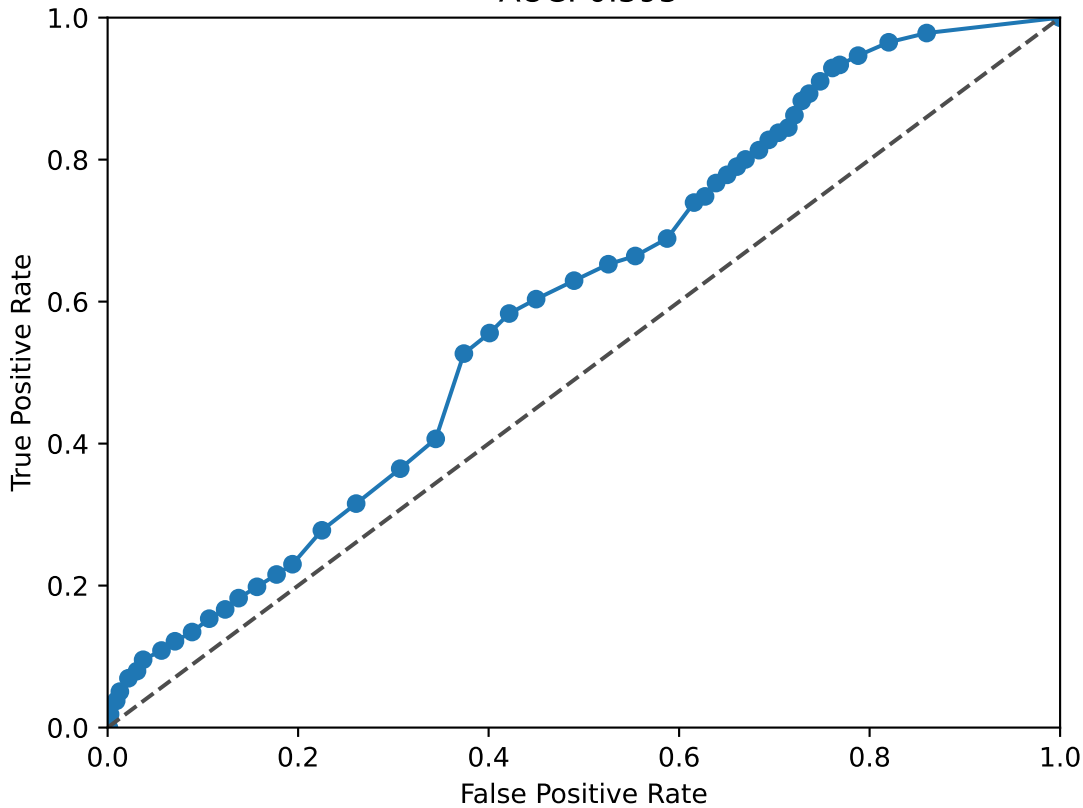
NFIA ROC Curve AUC: 0.595
