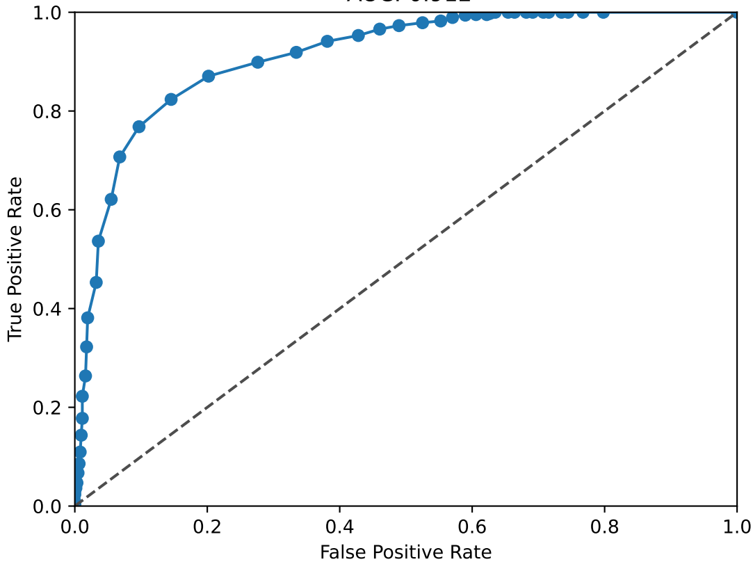
NFIB ROC Curve AUC: 0.912
