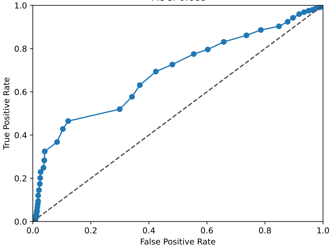
NFIX ROC Curve AUC: 0.689
