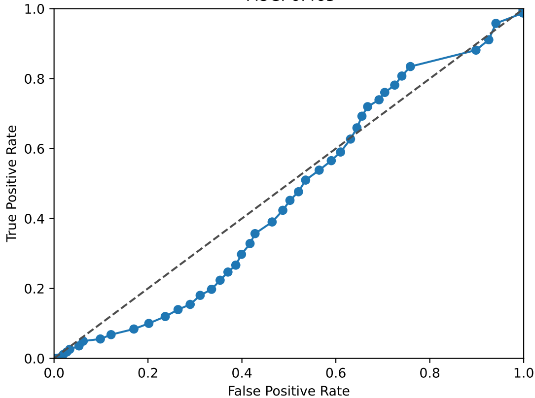
PKNOX2 ROC Curve AUC: 0.465
