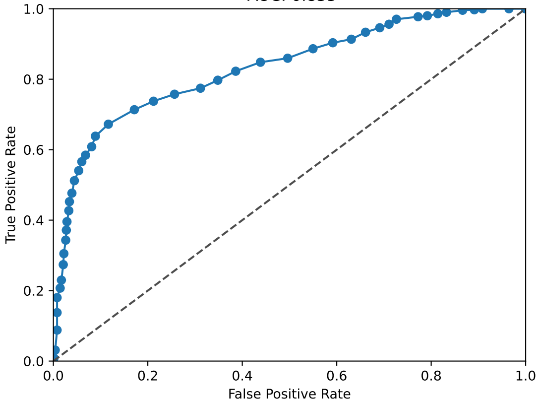
SIX4 ROC Curve AUC: 0.833
