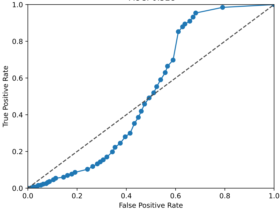
SOX11 ROC Curve AUC: 0.528
