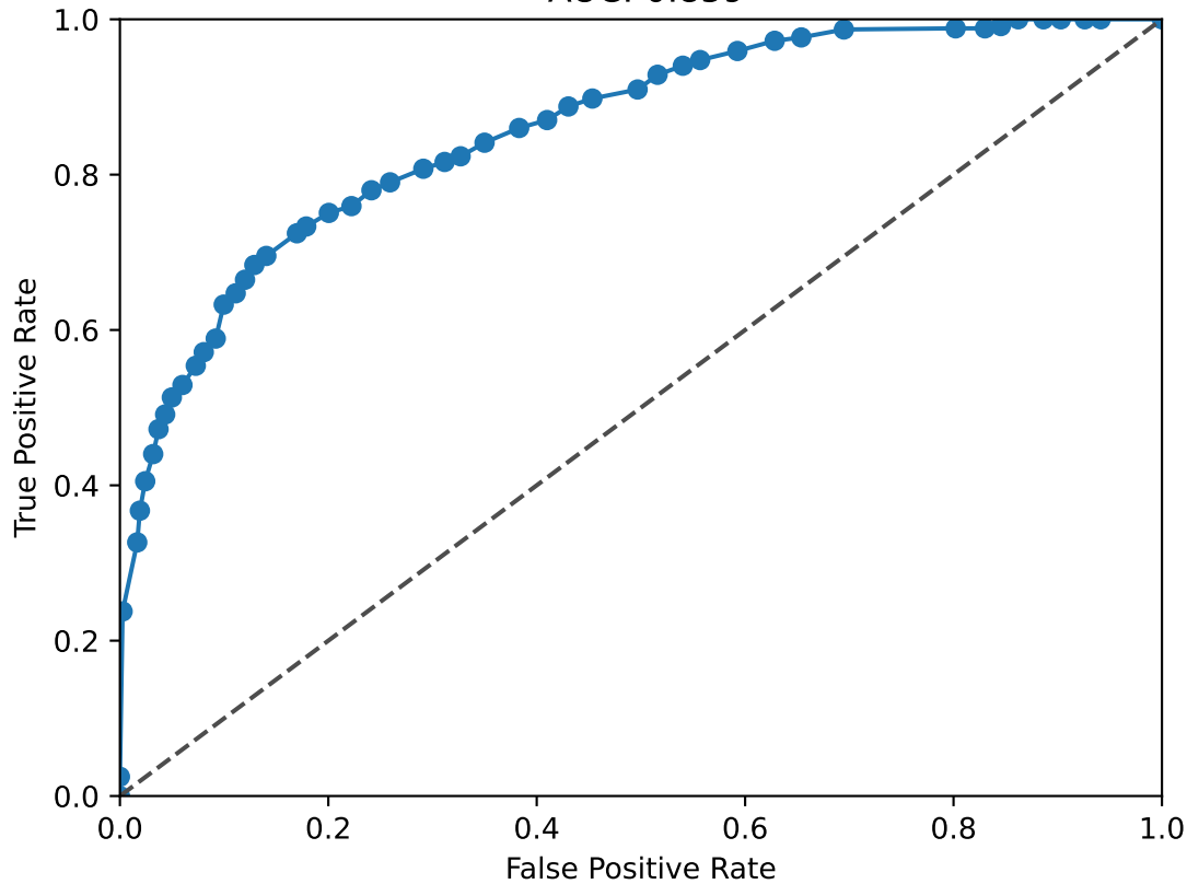
TEAD1 ROC Curve AUC: 0.859
