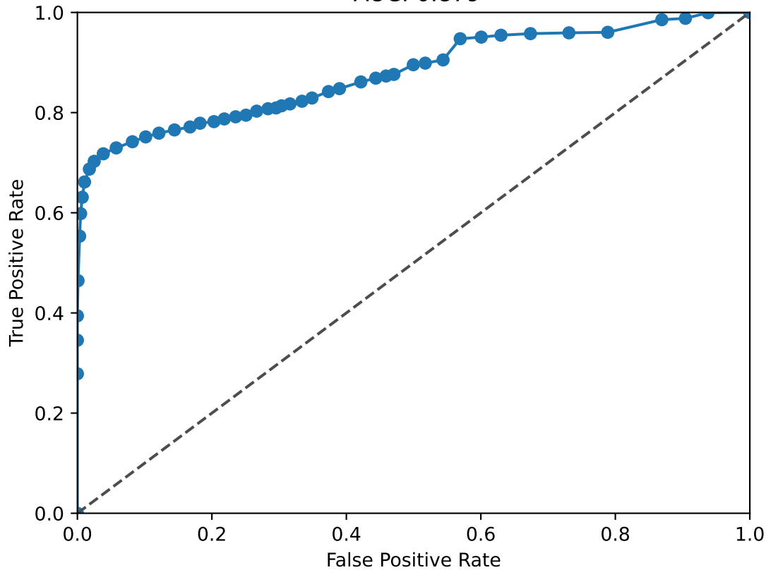
BACH1 ROC Curve AUC: 0.879
