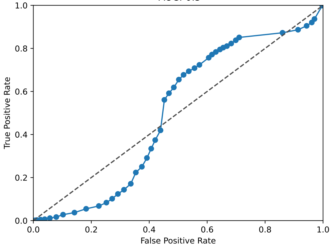
ETS1 ROC Curve AUC: 0.5
