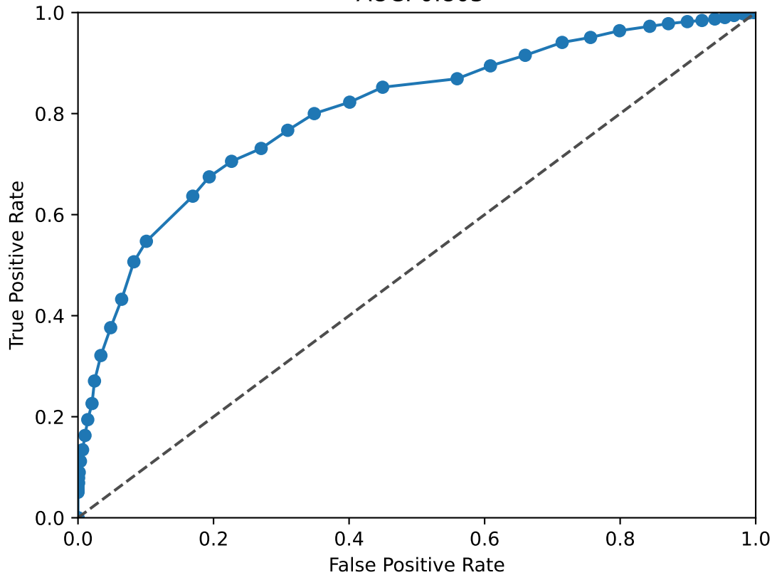
FOS ROC Curve AUC: 0.803
