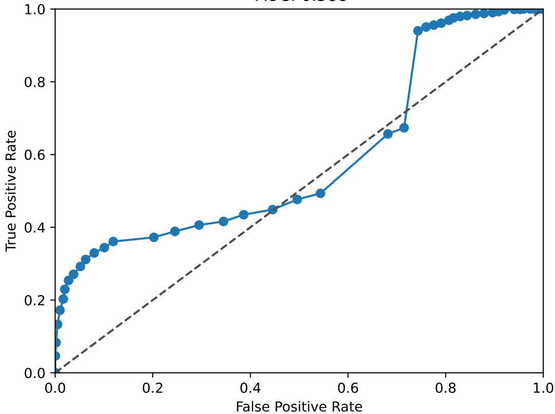
JUNB ROC Curve AUC: 0.588
