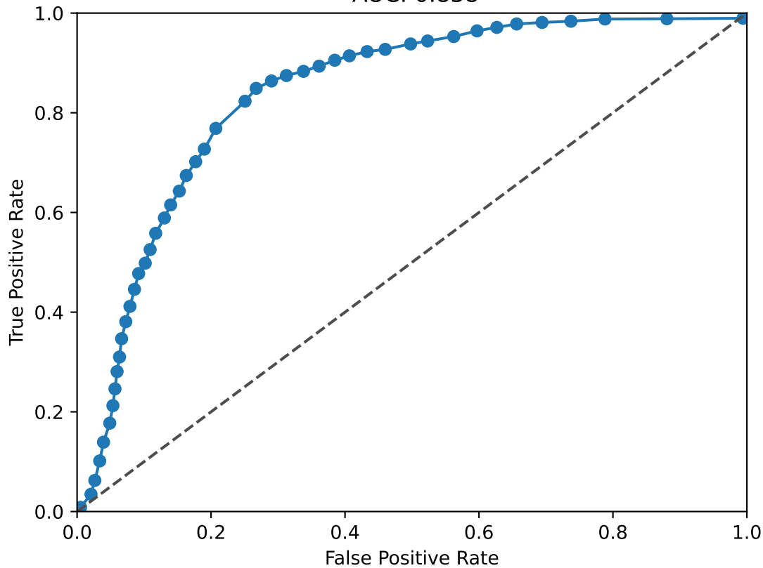
NCAM1 ROC Curve AUC: 0.838
