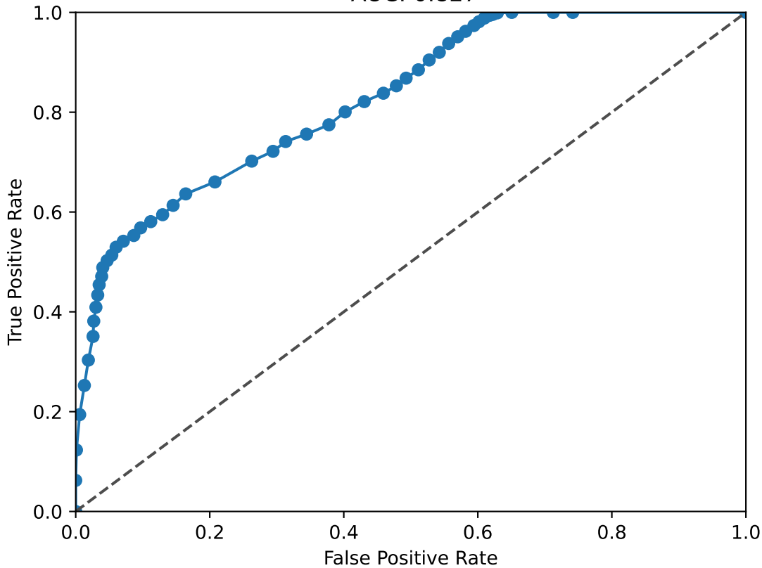
NFIB ROC Curve AUC: 0.827
