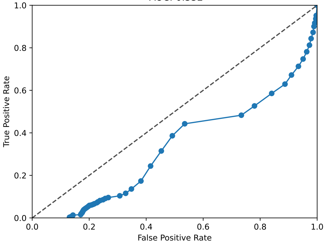
NFIX ROC Curve AUC: 0.332
