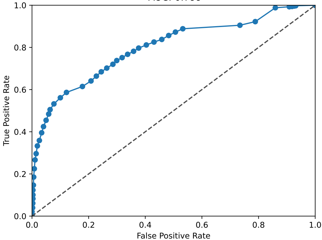
PKNOX2 ROC Curve AUC: 0.799
