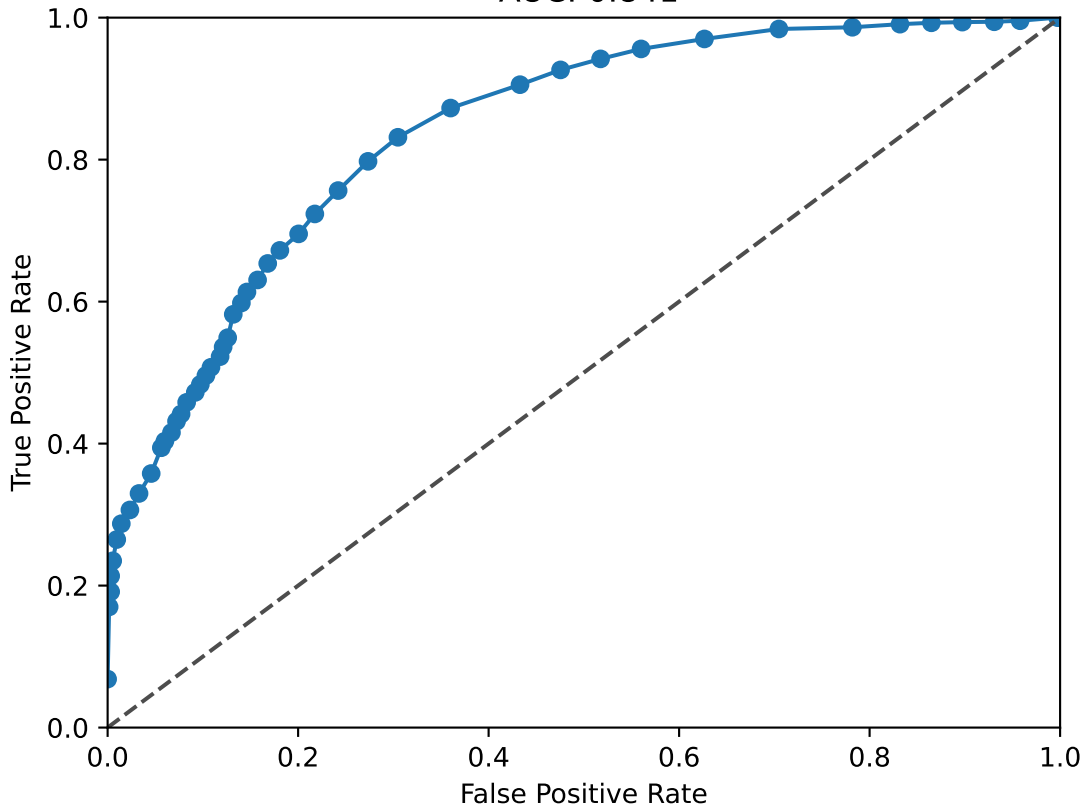
RUNX1 ROC Curve AUC: 0.841
