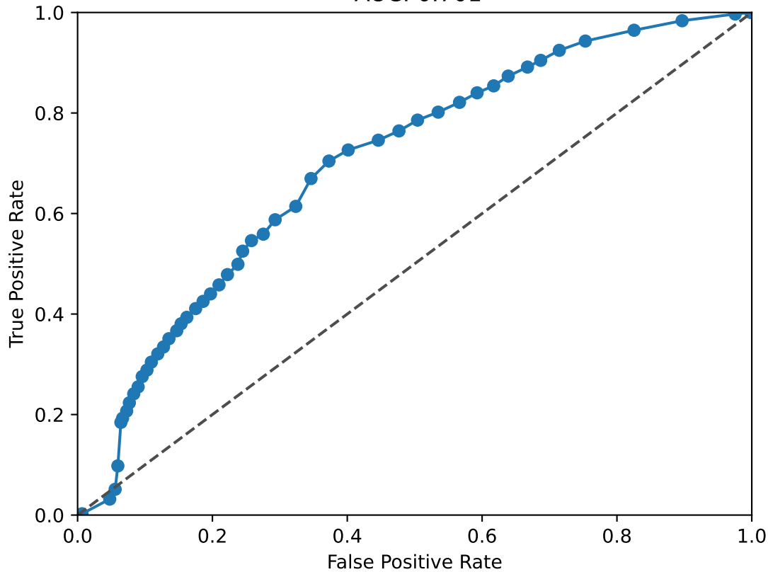
SMAD3 ROC Curve AUC: 0.701
