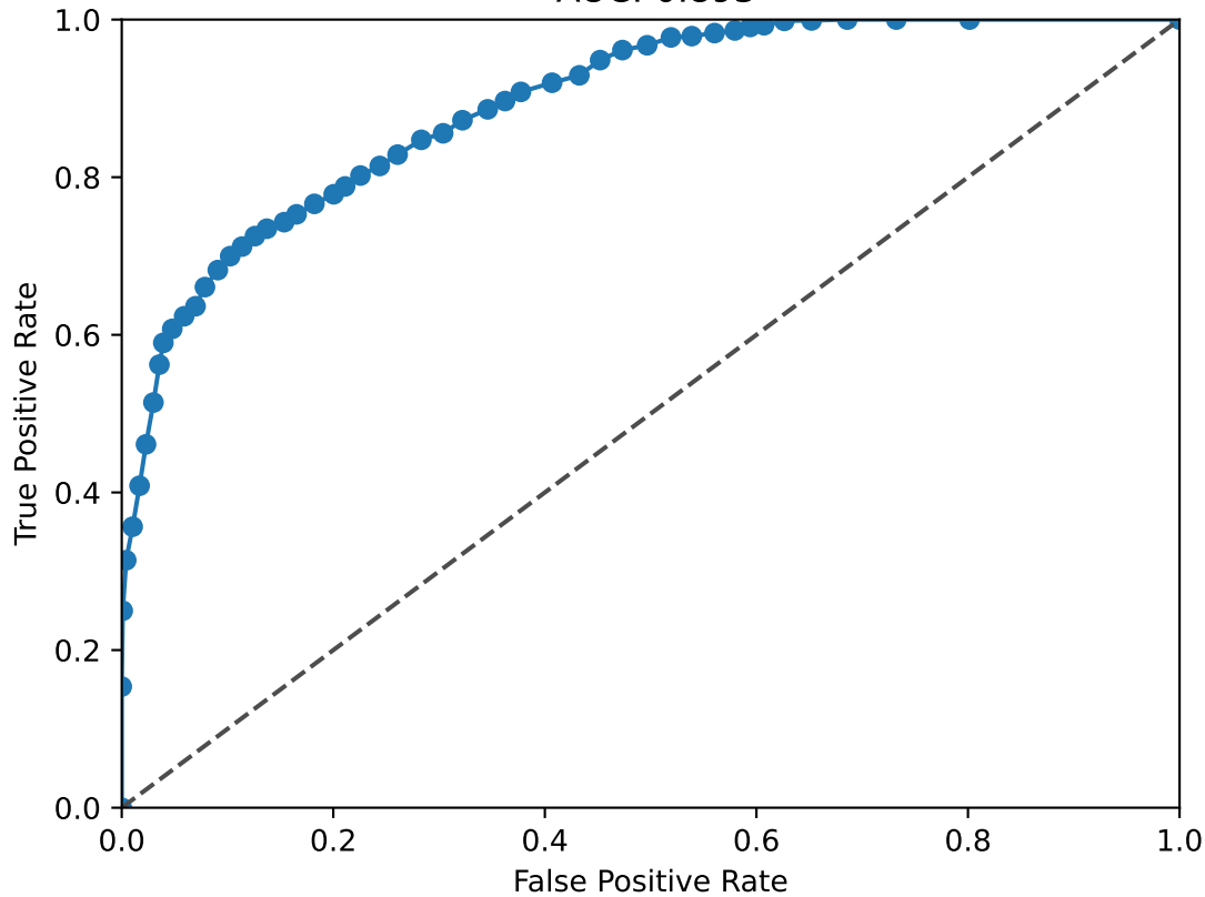
TEAD1 ROC Curve AUC: 0.893
