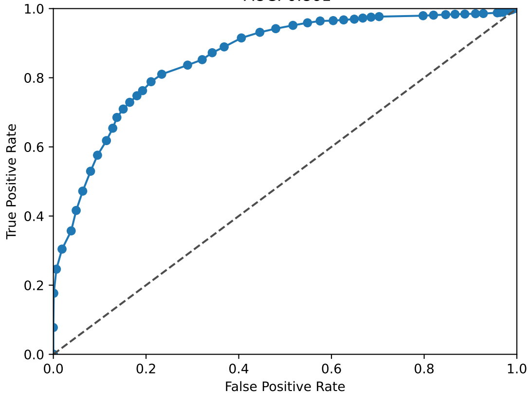
EGR1 ROC Curve AUC: 0.861
