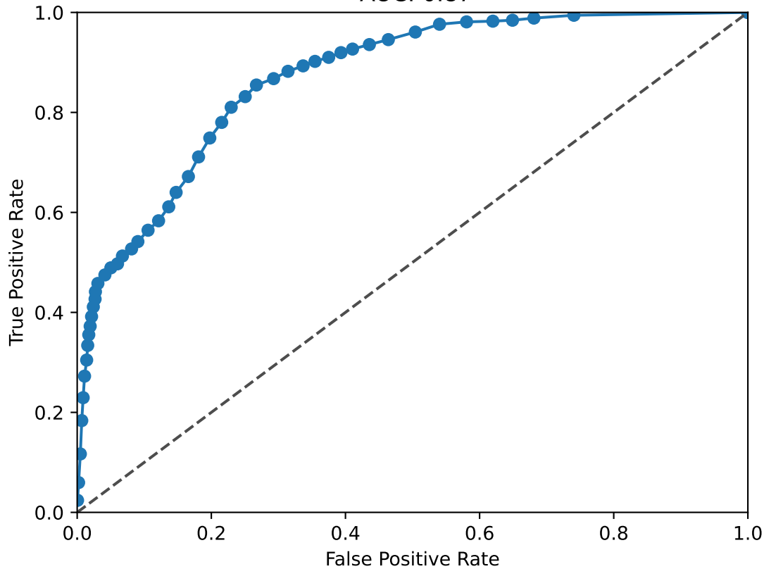
HSF2 ROC Curve AUC: 0.87
