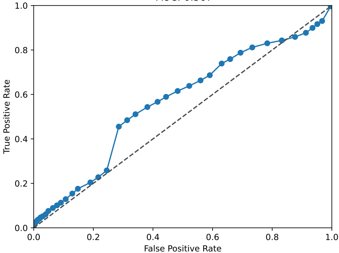
ICAM1 ROC Curve AUC: 0.567
