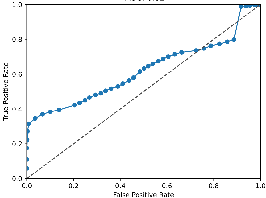
LMX1B ROC Curve AUC: 0.62
