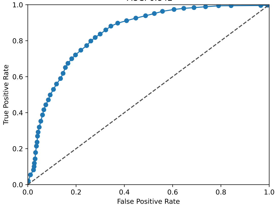
NCAM1 ROC Curve AUC: 0.842
