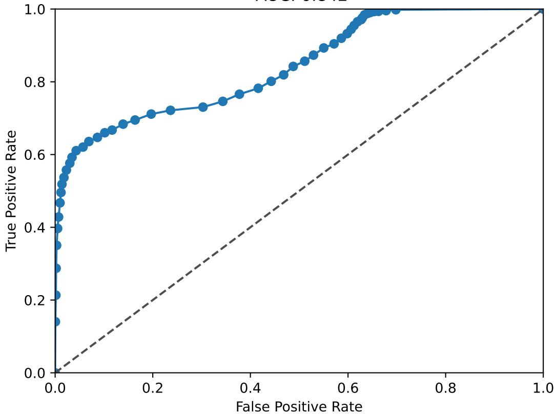
NFIB ROC Curve AUC: 0.842
