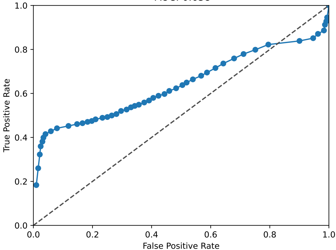
RORA_RORB ROC Curve AUC: 0.638
