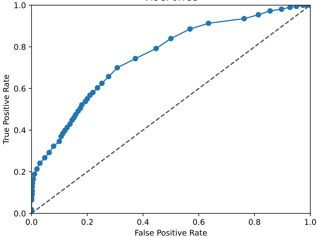
RUNX1 ROC Curve AUC: 0.755
