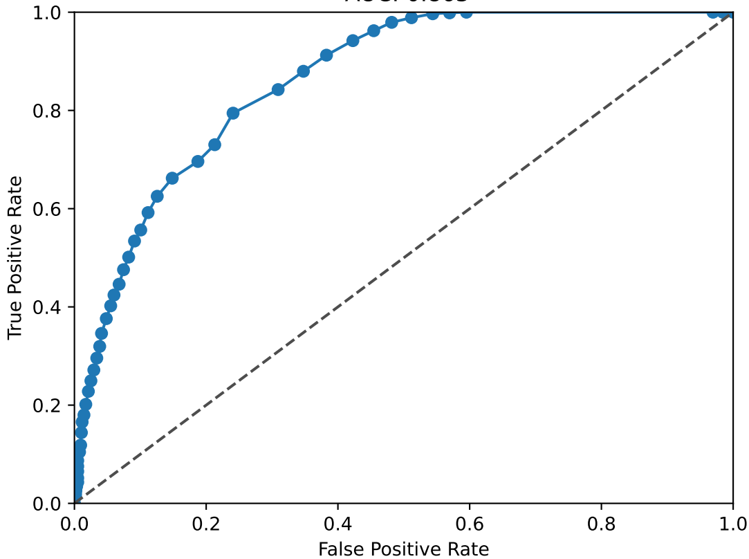
SIX1 ROC Curve AUC: 0.863
