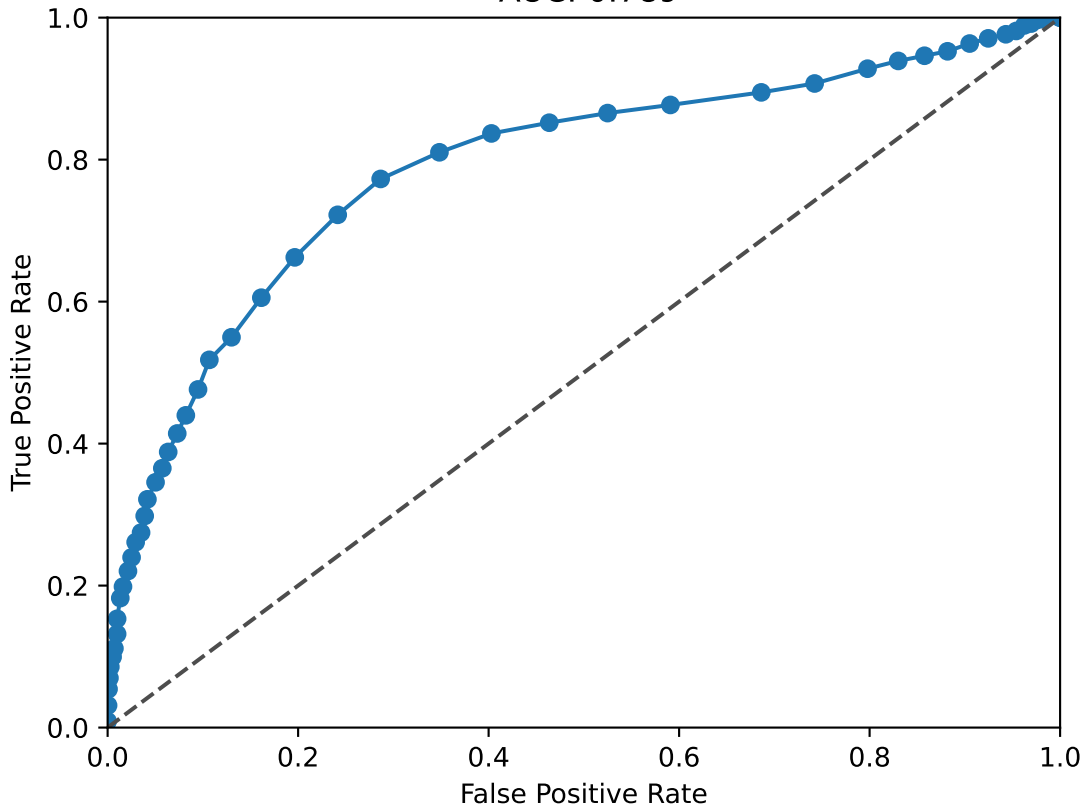
TCF7L1 ROC Curve AUC: 0.789
