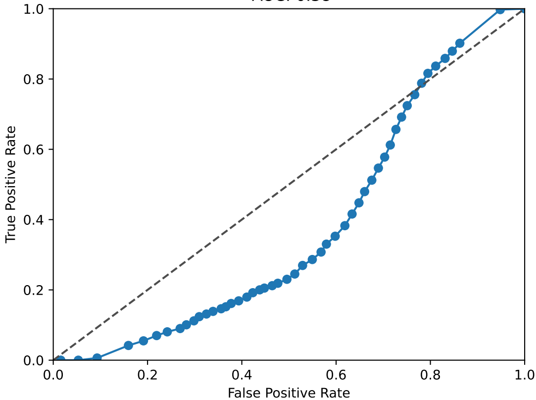
ASCL1 ROC Curve AUC: 0.38
