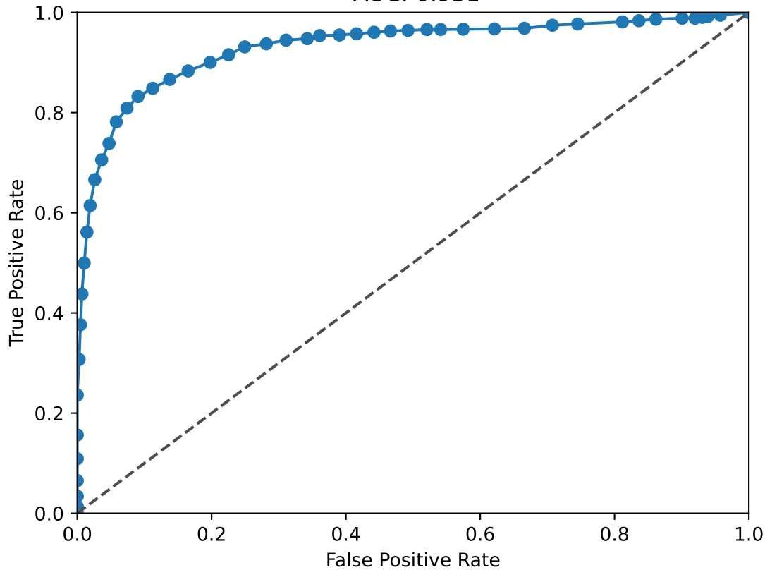
CUX2 ROC Curve AUC: 0.931
