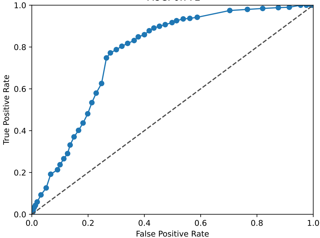
ETS1 ROC Curve AUC: 0.772
