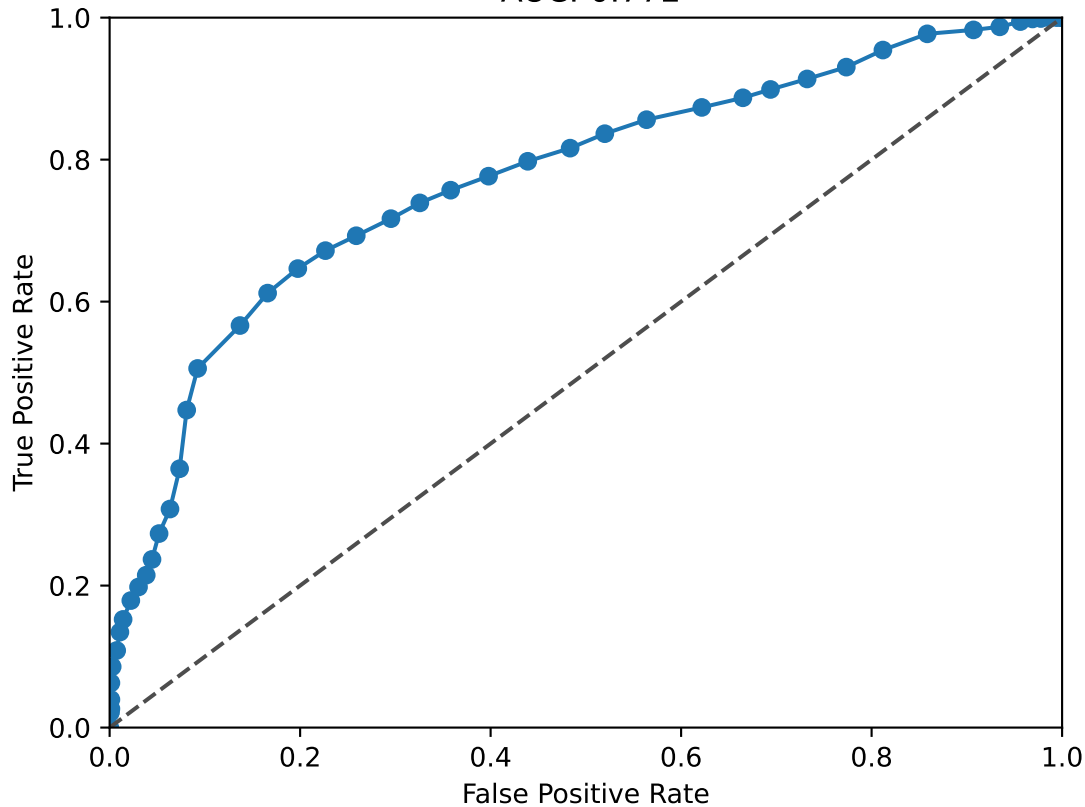
FOS ROC Curve AUC: 0.772
