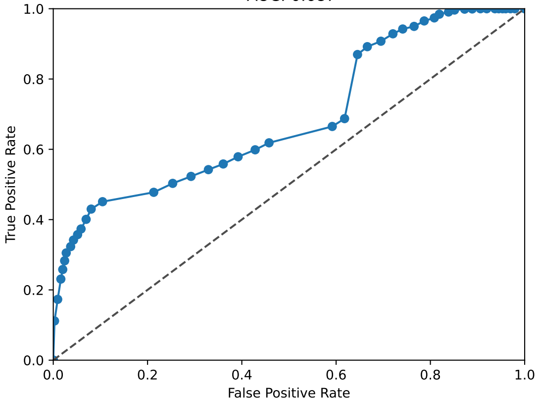
JUNB ROC Curve AUC: 0.687
