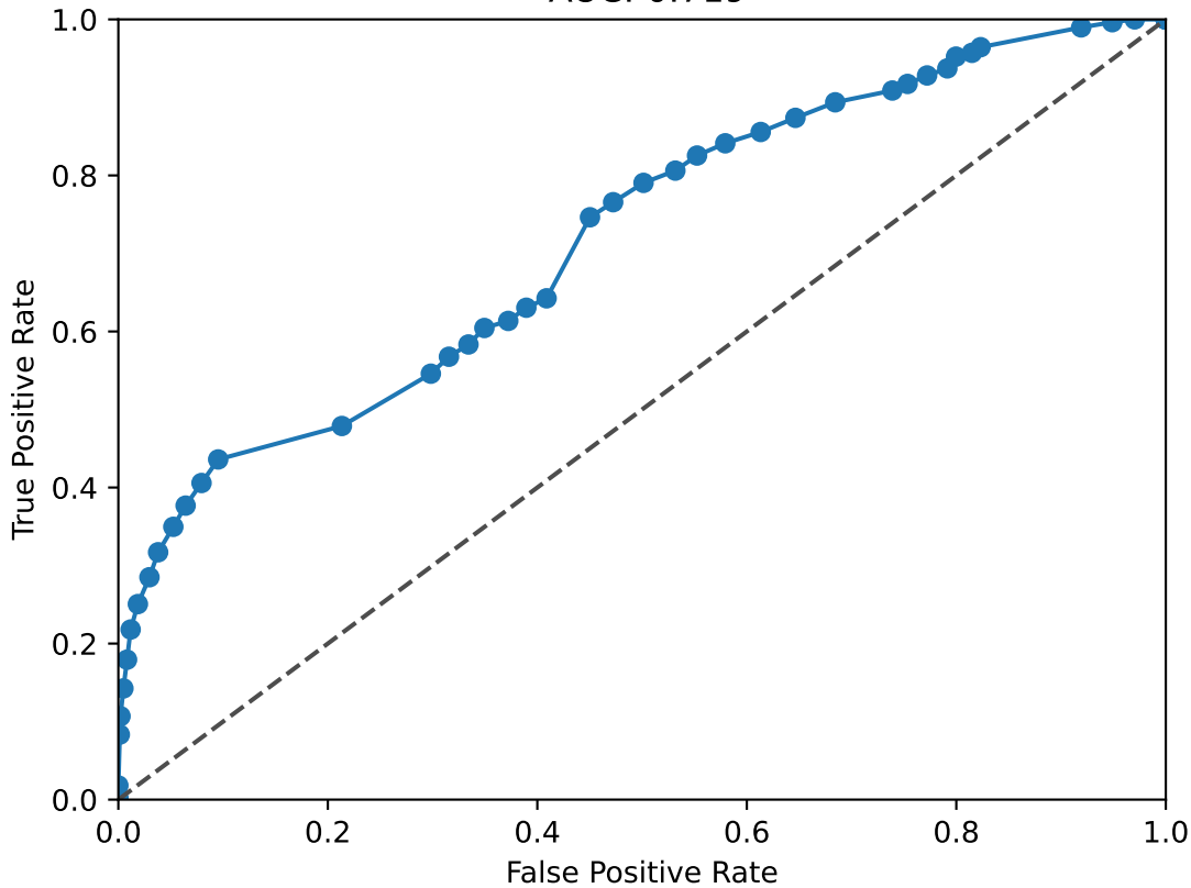
NFATC2 ROC Curve AUC: 0.719
