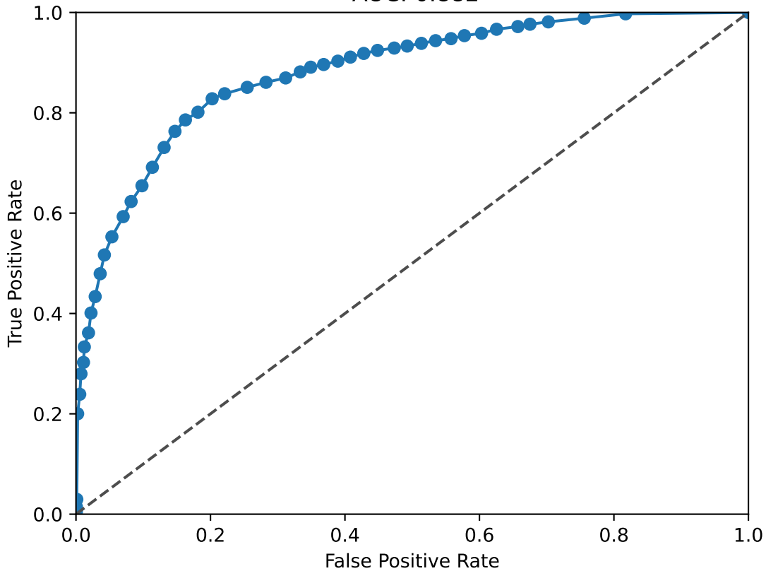
NFIA ROC Curve AUC: 0.882
