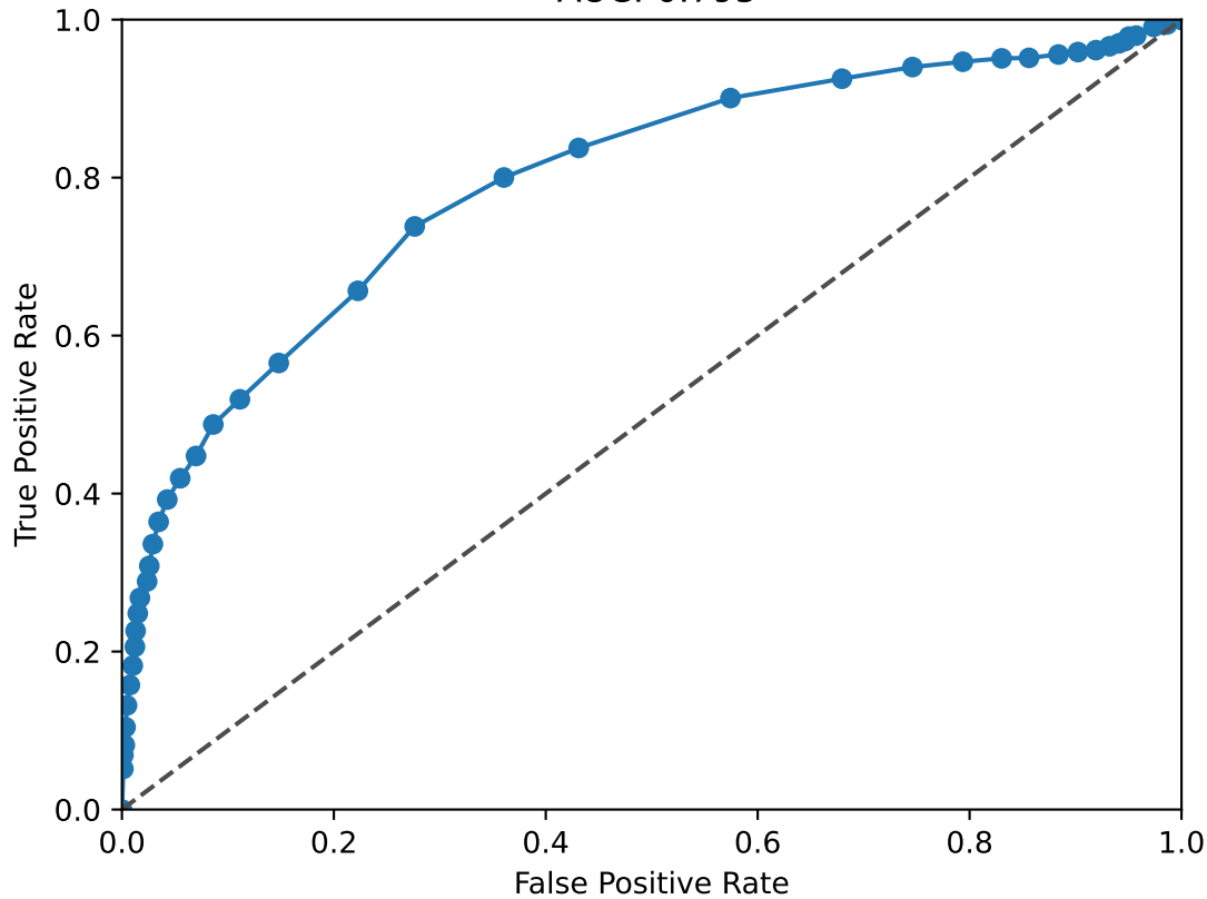
PBX1 ROC Curve AUC: 0.795
